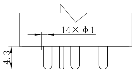
Pin Form "1"
