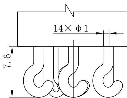
Pin Form "4"
